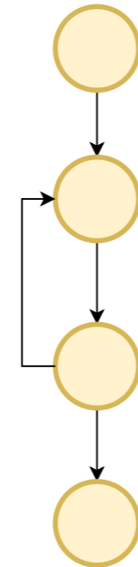
Do-while loop
