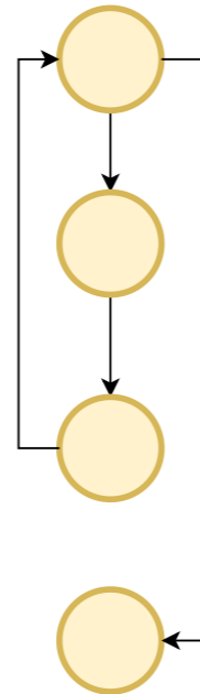
While loop
