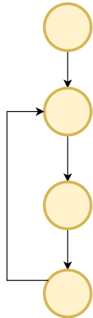
For loop
