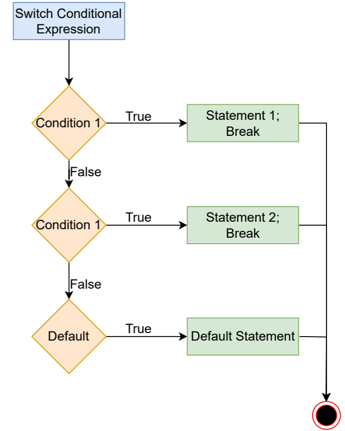
Switch case
